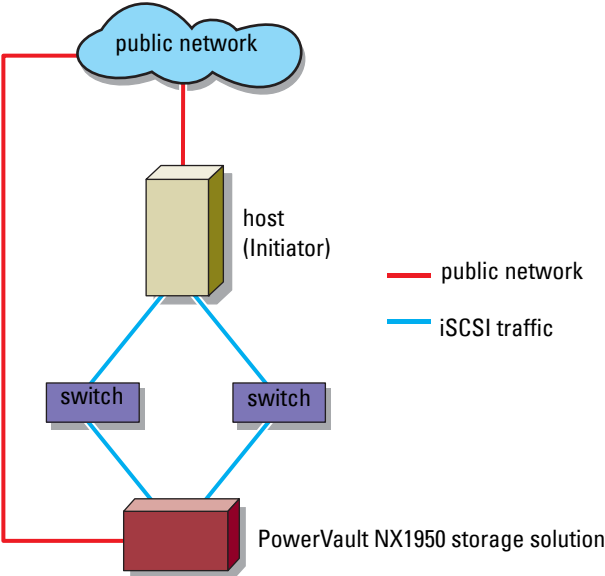
Figure 1-2. Redundant iSCSI Paths With Three NICs
