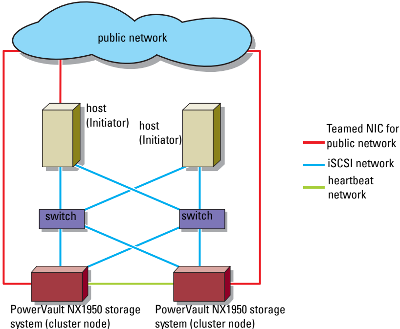
Figure 1-4. Redundant iSCSI Paths Using Four NICs
