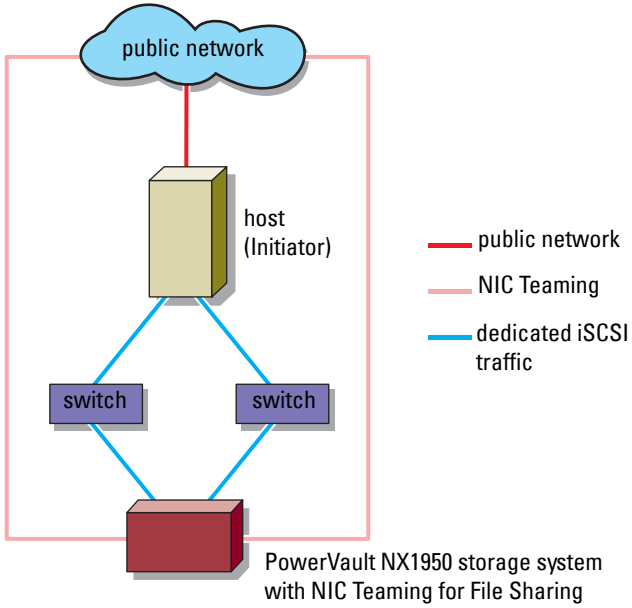
Figure 1-1. Redundant iSCSI Paths and NIC Teaming for Data Sharing With Four NICs
