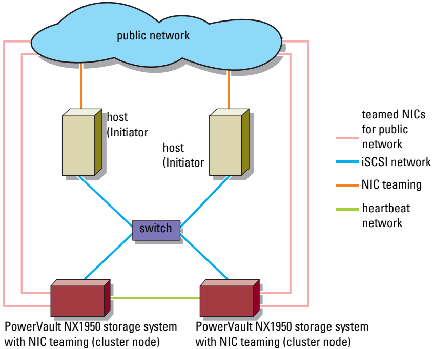
Figure 1-5. Non-Redundant iSCSI Paths Using Four NICs
