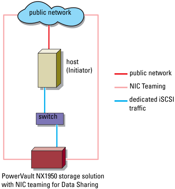
Figure 1-3. Non-Redundant iSCSI Path With Three NICs
